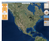
Dashboard
