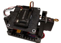
Gimbal Kit
